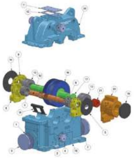
Increasing & Reducing Gears (Philadelphia Gear, USA)
